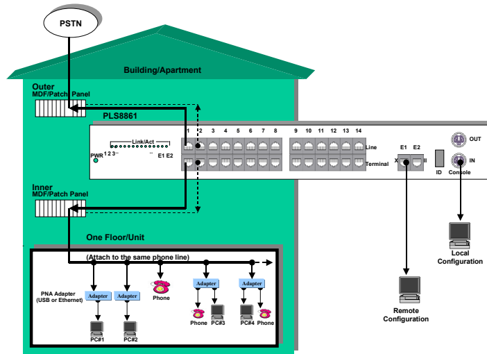
Figure 2 Cabling of one PLS8860/PLS8861
