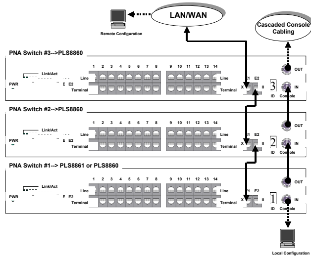
Figure 3 Cabling of more PLS8860/PLS8861
