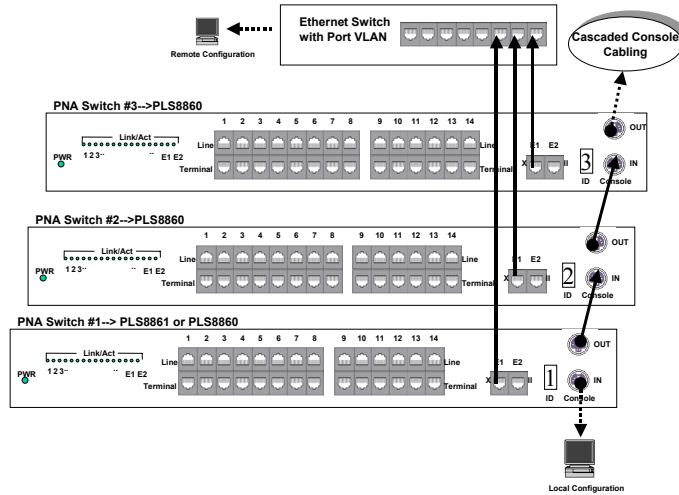
Figure 4 Cabling of more PLS8860/PLS8861 by Ethernet Switch
